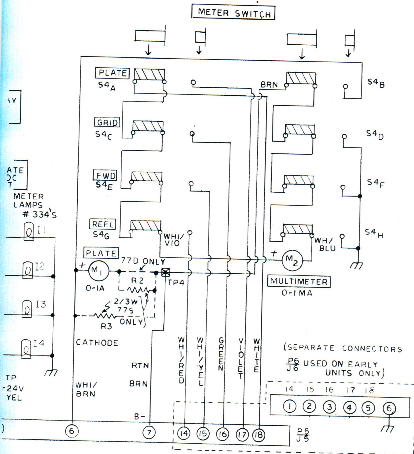
FIG. 20: ALPHA 77D & 77S SCHEMATIC - FRONT PANEL
